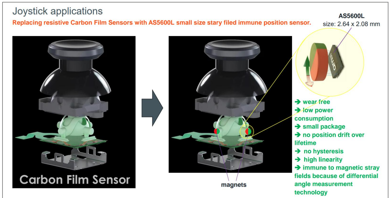
Figure 1: Joystick applications
